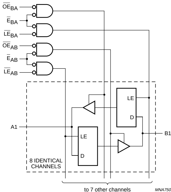
Fig.5 Logic diagram.
